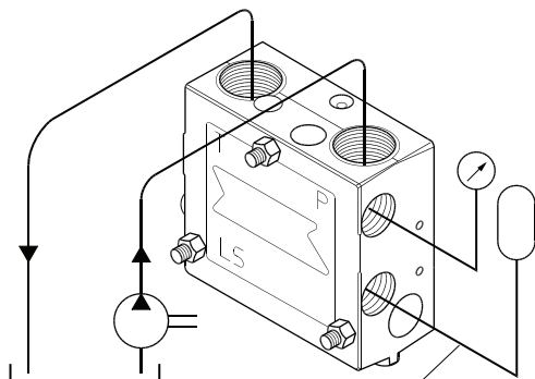
Accumulator port
