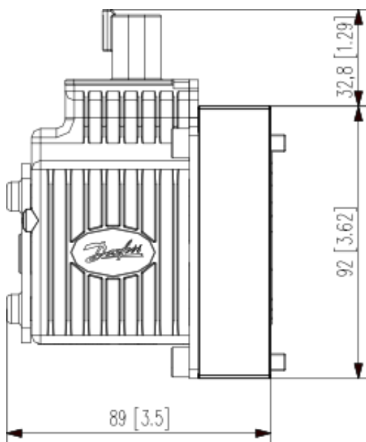
PVEA Series 7 dimensions
